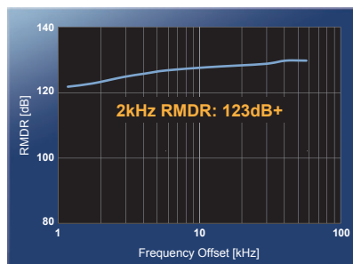
■ 14MHz Band Reciprocal Mixing Dynamic Range (RMDR)
