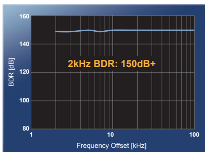
■ 14MHz Band Blocking Dynamic Range (BDR)
