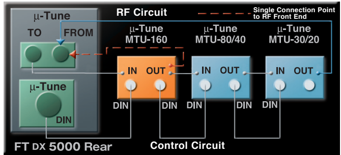
■ RF \mu -Tune unit Connection Diagram
